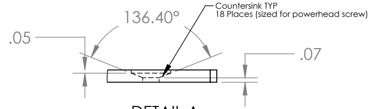
DETAIL A SCALE 1 : 1.5
